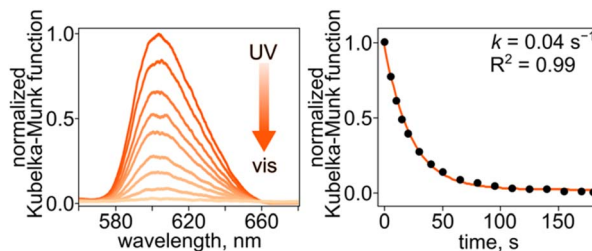
Fig. 9 (Left) diffuse reflectance spectra of UiO-67 + SP-COOH upon exposure to a 365 nm excitation wavelength for 30 s followed by exposure to white light ( \lambda_{\text{ex}} = 400\text{--}900 nm). The gradient from orange to yellow indicates photoisomerization from the merocyanine to spiropyran isomers. (Right) plot demonstrating the change in absorbance of UiO-67 + SP-COOH after exposure to a 365 nm excitation wavelength for 30 s followed by exposure to white light ( \lambda_{\text{ex}} = 400\text{--}900 nm). Data fitting (orange line) with a first-order exponential decay equation resulted in a photoisomerization rate constant ( k ) of 0.04 \text{ s}^{-1} .
