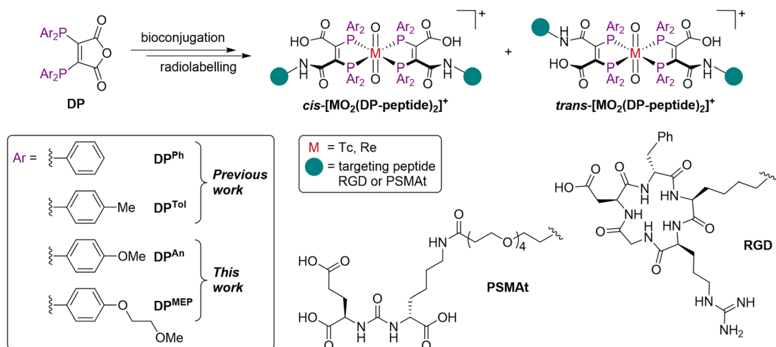
Fig. 1 Structures of cis/trans - [\text{MO}_2(\text{DP-peptide})_2]^+ complexes, where M = \text{Tc} or \text{Re} . 18–20
