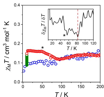
Fig. 7 Plot of \chi_M T vs. T for 4 \cdot 1.7^1\text{Pr}_2\text{O} upon cooling (blue circles) response with irradiation with 420 nm for 12 hours at 10 \text{ K} (green circles), and subsequent warming scan after the light is switched off (red circles). Inset figure shows \delta\chi_M T / \delta T vs. T , with T(\text{photoirradiation}) indicated by the red line ( 82 \text{ K} ). * Bump due to molecular oxygen.
