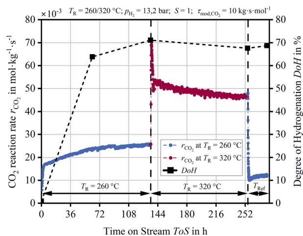
Fig. 5 r_{\text{CO}_2} and \text{DoH} over \text{ToS} for quantification of the loss of catalytic activity for steady-state operation.
