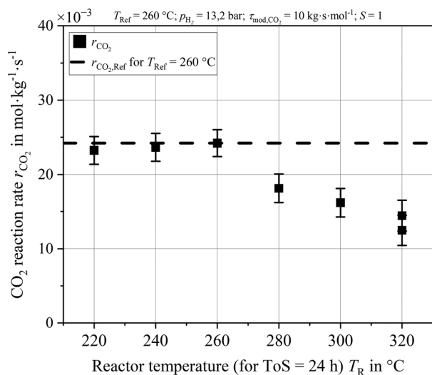
Fig. 4 r_{\text{CO}_2} at T_{\text{Ref}} = 260\text{ }^{\circ}\text{C} after three-phase \text{CO}_2 methanation at different T_R for \text{ToS} = 24\text{ h} ; data provided by ref. 38.
