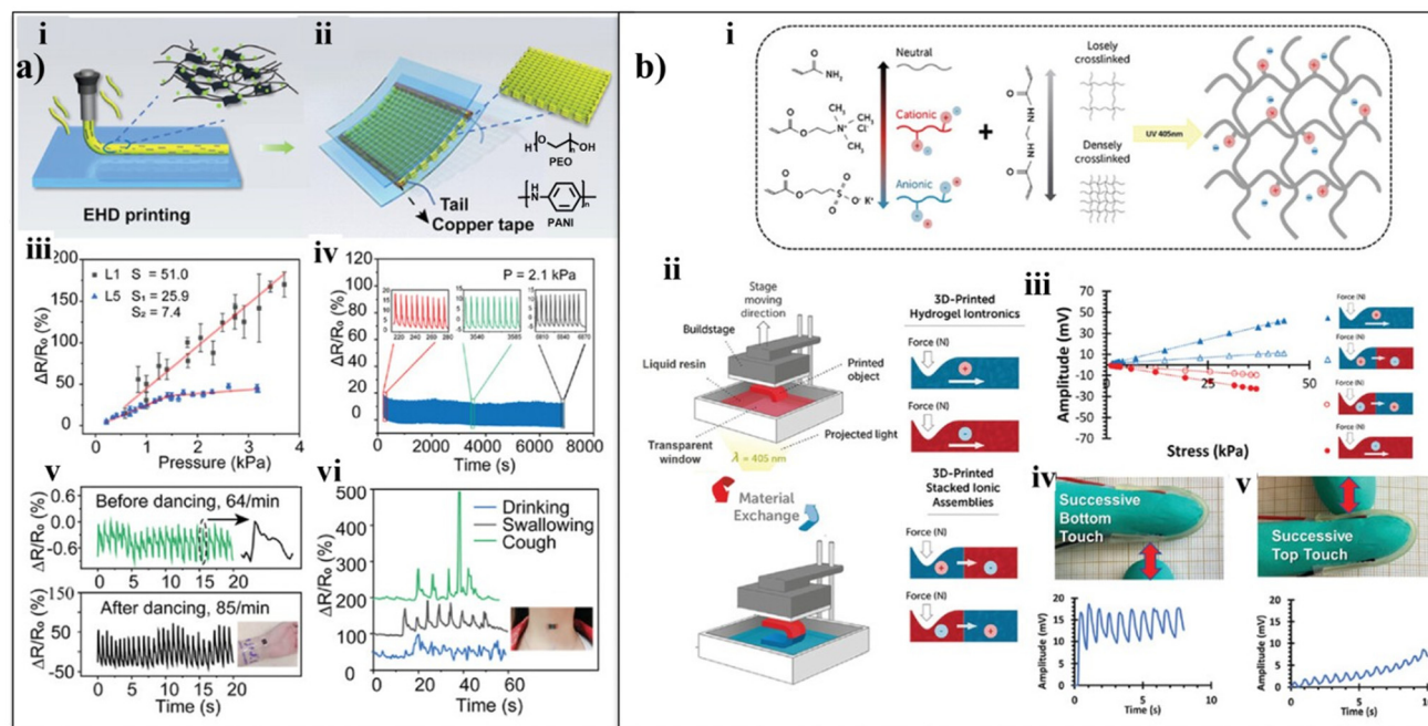
Fig. 16 (a) (i) EHD jetting was used to deposit a sensing layer composed of PEO, PANI, and graphene. (ii) Illustration showing the cross-sectional structure of the completed layered pressure sensor. (iii) Sensor resistance variation under applied pressure for configurations with one and five jetted layers. (iv) Stability of the sensor's resistance over 1000 cycles of loading and unloading at a 0.15 Hz frequency. (v) Detection of pulse waveforms captured by the sensor both before and after physical exercise (dancing). (vi) Resistance signal profiles corresponding to human actions such as coughing, swallowing, and drinking. Reproduced with permission from ref. 206. Copyright 2022, ACS. (b) (i) Schematic of the copolymerization reaction involving AAm with either AETA or SPA, using MBA as the crosslinker, utilized in SLA printing. (ii) Demonstration of SLA-based fabrication of multilayered ionic structures through alternating resin vats, enabling control over ionic species, charge densities, and crosslinking levels within the iontronic components. (iii) Voltage output response as a function of stress applied to compartments containing either SPA or AETA at 30 mol% concentration. (iv and v) A 3D-printed dual-compartment finger sleeve mimicking tactile responses at the fingertip and fingernail, exhibiting distinct sensitivity profiles. Reproduced with permission from ref. 207. Copyright 2023, Wiley.
