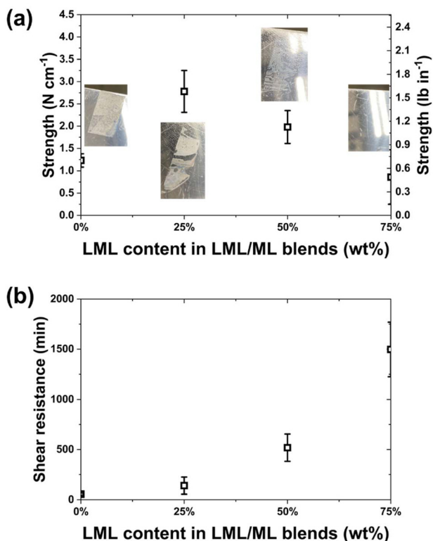
Fig. 7 (a) 180^\circ peel adhesion properties and (b) shear resistance properties on stainless steel substrates of alkyne-ML(38.8, 0.26) and LML/ML blends after solvent casting with additional 20 wt% tackifier. All of the 180^\circ peel adhesion tests were performed at the rate of 305 \text{ mm min}^{-1} . Inserted digital images in (a) show the stainless steel substrate surfaces after the 180^\circ peel adhesion tests.
