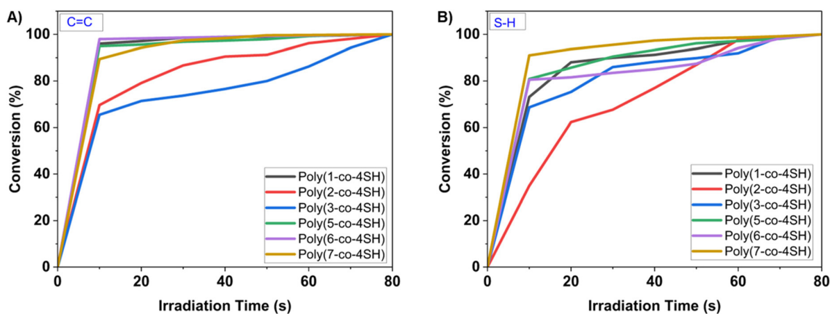
Fig. 2 Percentage conversion vs. irradiation time: (A) alkene (C=C) and (B) thiol (S–H), for all six thermosets, based on FTIR analysis during UV irradiation.
