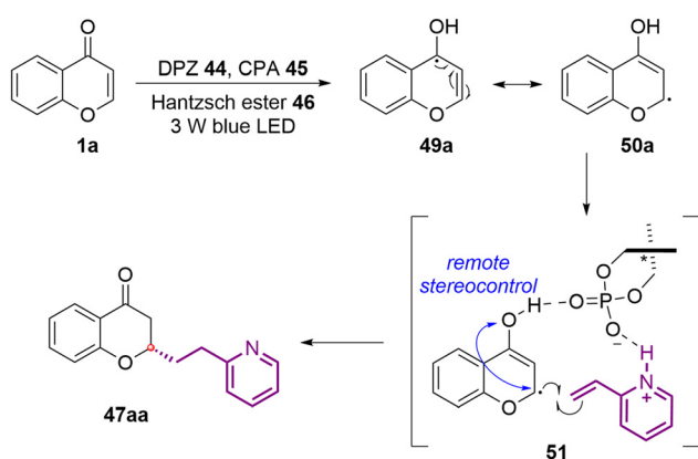
Scheme 15 Proposed mechanism through radical intermediates.
