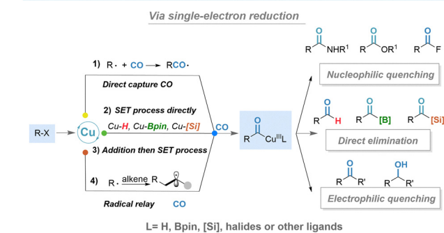
Fig. 2 Diverse types of single-electron reduction processes of organic halides.
