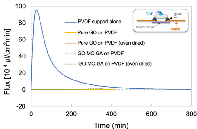
Fig. 6 Diethyl chlorophosphate (DCP) permeation rates through GO (3 μm) and GO–MC–GA (10 μm) films under conditions of vapor-only contact. All films are supported on a porous PVDF filter during testing, which allows rapid DCP vapor permeation when used alone as a positive control. All films studied here are effective DCP vapor barriers.
