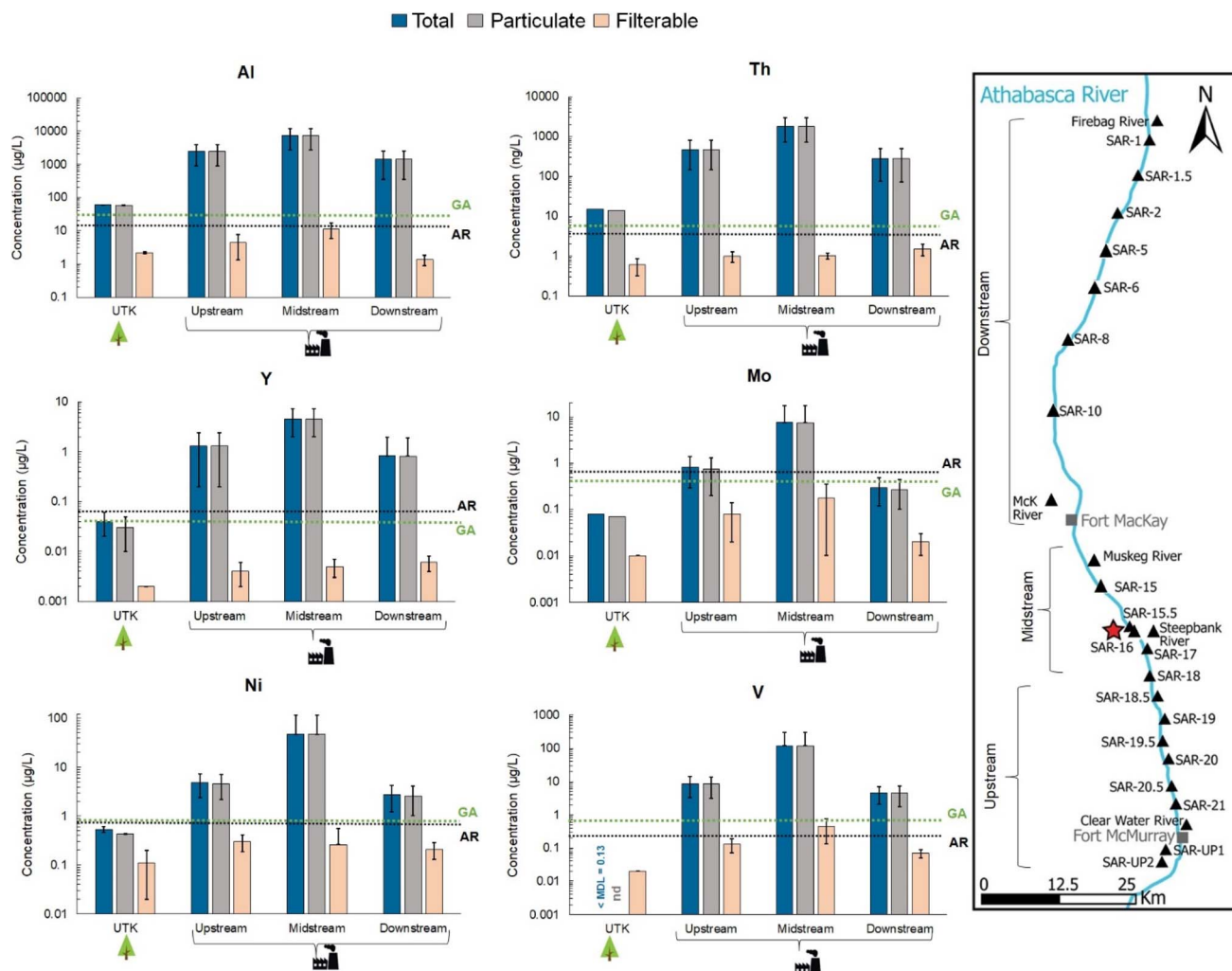
Fig. 2 Average concentrations of total, particulate and filterable (<0.45 µm) Al, Th, Y (conservative lithophile elements), Mo, Ni, and V (elements enriched in bitumen) in snow from upstream, midstream, and downstream locations (with respect to the industry), and at the reference site (UTK), winter 2016. The horizontal black line represents the dissolved TE concentrations in the AR main stem in autumn of 2014 (ref. 36) whereas the green line represents the global average (GA) dissolved (<0.2 or 0.45 µm) concentrations of TEs in river water. 64 Notes: the map on the right side shows the snow sampling locations in the ABS region along the Athabasca River (SAR) and its tributaries. The location of UTK is provided in Fig. S1 and Table S1 (SI). The red star represents the midpoint between bitumen upgraders. Error bars represent one standard deviation. LOD = limit of detection, MDL = method detection limit, nd = not determined. Th and Mo concentrations at UTK are based on one location instead of the average of two.
