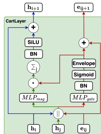
Fig. 9 Schematic of the CartLayer used in CartNet. This layer aggregates information between two neighbouring atoms, the sender atom \mathbf{h}_i^t and the receiver atom \mathbf{h}_j^t , and their corresponding edge, \mathbf{e}_{ij}^t . It utilizes this aggregated information to update the receiving node's features and the edge's latent vector. The updated receiving node, \mathbf{h}_i^{t+1} and the respective edge, \mathbf{e}_{ij}^{t+1} , representations are then propagated to subsequent layers for further processing.
