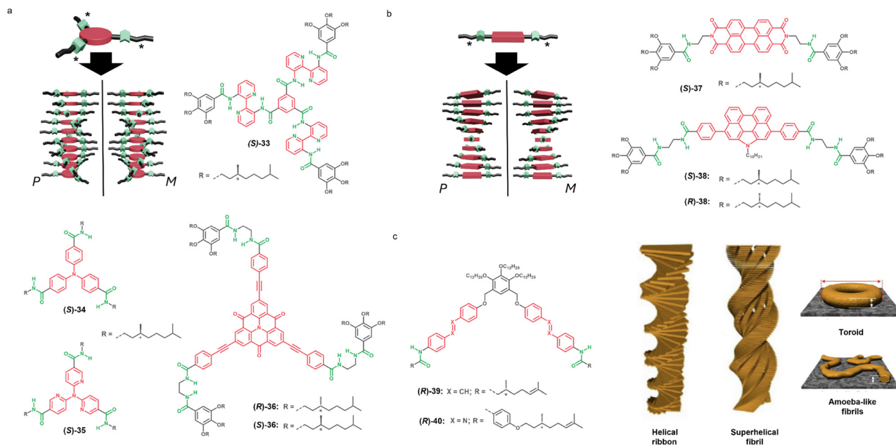
Fig. 12 (a) Schematic representation of the asymmetry transfer in C_3 -symmetry scaffolds upon aggregation by point chirality and BTA ( S-33 ), triaryl amines ( S-34 and S-35 ) and N-heterotriangulenes ( S-36 and R-36 ) chemical structures. (b) Schematic representation of C_2 -symmetry monomer chiral self-assembly and chemical structure for chiral PBI ( S-37 ) and chiral N-annulated perylenes ( S-38 and R-38 ) (c) Chemical structures of scissor-shaped monomers endowed with point chirality ( R-39 and R-40 ) employed by S. Yagai and coworkers and schematic representation of different supramolecular aggregates than can be observed in the supramolecular polymerization process ( R-39 ) depending on the molar fraction of the cross-linked specie, namely: helical ribbon, superhelical fibril, toroid and amoeba-like fibrils (reproduced from ref. 196, with permission of Springer Nature, copyright 2015).
