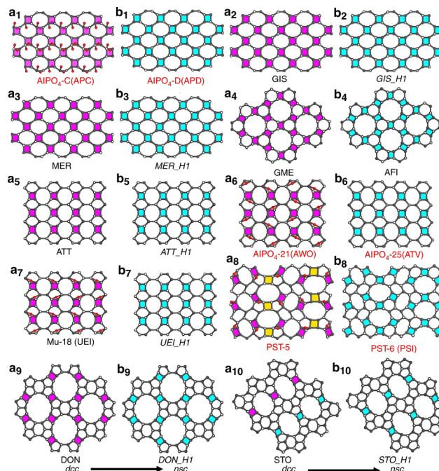
Fig. 16 Zeolite and AlPO frameworks (a 1 )–(a 10 ) transferred into (b 1 )–(b 10 ) frameworks by changing dcc to narsarsukite ( nsc ) chains. 292 Magenta: dcc ; cyan: nsc ; yellow: double four-ring (d4r). Reproduced from ref. 292 under CC-BY-4.0 licence https://creativecommons.org/licenses/by/4.0/ .
