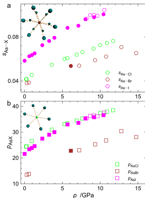
Fig. 3 As \cdots X bond valences (a) and penetration indices (b) plotted as a function of pressure for the studied intercalation compounds. Insets present \text{Br}^- (a) and \text{Cl}^- (b) anions interacting with twelve As atoms in P_{\text{NH}_4\text{Br}} and six As atoms Y_{\text{NH}_4\text{Cl}} , respectively.
