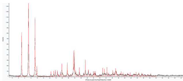
Fig. 4 PXRD of the new AgSD-NO 3 (black) compared with the theoretical pattern (red).
