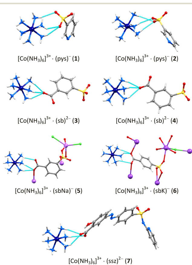
Fig. 9 View of the selected pairs for the estimation of their interaction energies.
