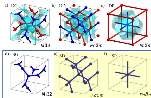
Figure 1. (a-c) Double network cubic phases with corresponding space groups and their infinite minimal surfaces (blue) and (d-f) the corresponding single networks. Reproduced from ref. 16.
