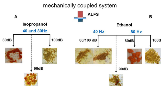
Fig. 4 Mechanically coupled crystallisations: (A) ROY polymorphs formed in isopropanol at different sound amplitudes regardless frequency, (B) ROY forms obtained in ethanol in which sound frequency and amplitude prove to be significant parameters; dashed lines indicate concomitant crystallisation.
