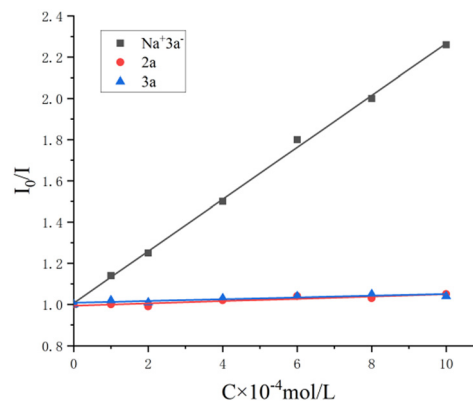
Fig. 1 Stern–Volmer plots. I 0 is the inherent fluorescence intensity of [Ir(ppy) 3 ](ppy) 2 PF 6 . I is the fluorescence intensity of [Ir(ppy) 3 ](ppy) 2 PF 6 in the presence of Na + 3a − , 2a or 3a .
