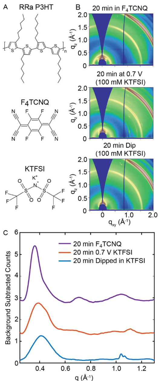
Fig. 1 2D GIWAXS diffractograms and radially integrated diffractograms of RRa P3HT under different conditions. (A) Chemical structures of RRa P3HT, F 4 TCNQ, and KTFSI. (B) GIWAXS diffractograms of a RRa P3HT thin film immersed in 10 mg mL −1 F 4 TCNQ for 20 min (top), doped at 0.7 V vs. Ag/AgCl for 20 min (middle), and immersed in an aqueous 100 mM KTFSI electrolyte for 20 min (bottom). (C) Radially integrated and background subtracted GIWAXS diffractograms of the RRa P3HT thin films.
