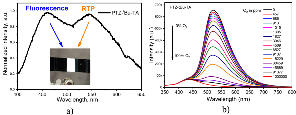
Fig. 22 Electroluminescence (EL) spectra of host-free devices based on the organic RTP emitter PTZ-tBu-TA (a) and PL spectra of PTZ-tBu-TA dispersed in the PMMA matrix at different concentrations of oxygen (b). Reprinted from K. Leitonas, A. Tomkeviciene, G. Baratte, A. Dabulienė, S. M. Punniyakoti, D. Volyniuk and J. Vidas Grazulevičius, oxygen sensing properties of thianthrene and phenothiazine derivatives exhibiting room-temperature phosphorescence: Effect of substitution of phenothiazine moieties, Sens. Actuators, B , 345 , 130369, 102 Copyright 2023, with permission from Elsevier.
