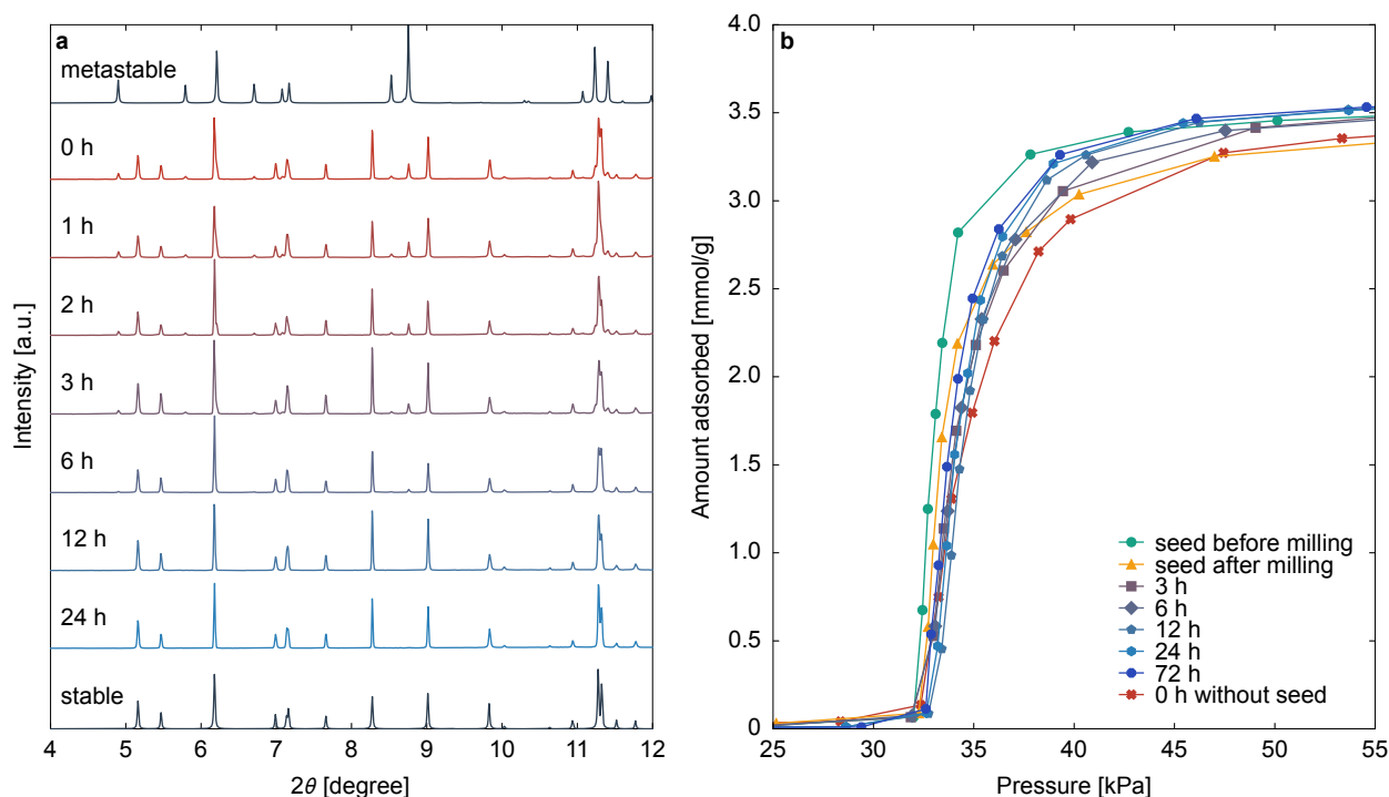
Fig. 7 Changes in (a) the XRD pattern of pre-ELM-11 and (b) the CO 2 adsorption isotherm on ELM-11 at 273 K when varying the aging time during synthesis with the addition of seeds. The XRD patterns were measured at \lambda = 0.0799932 nm.
