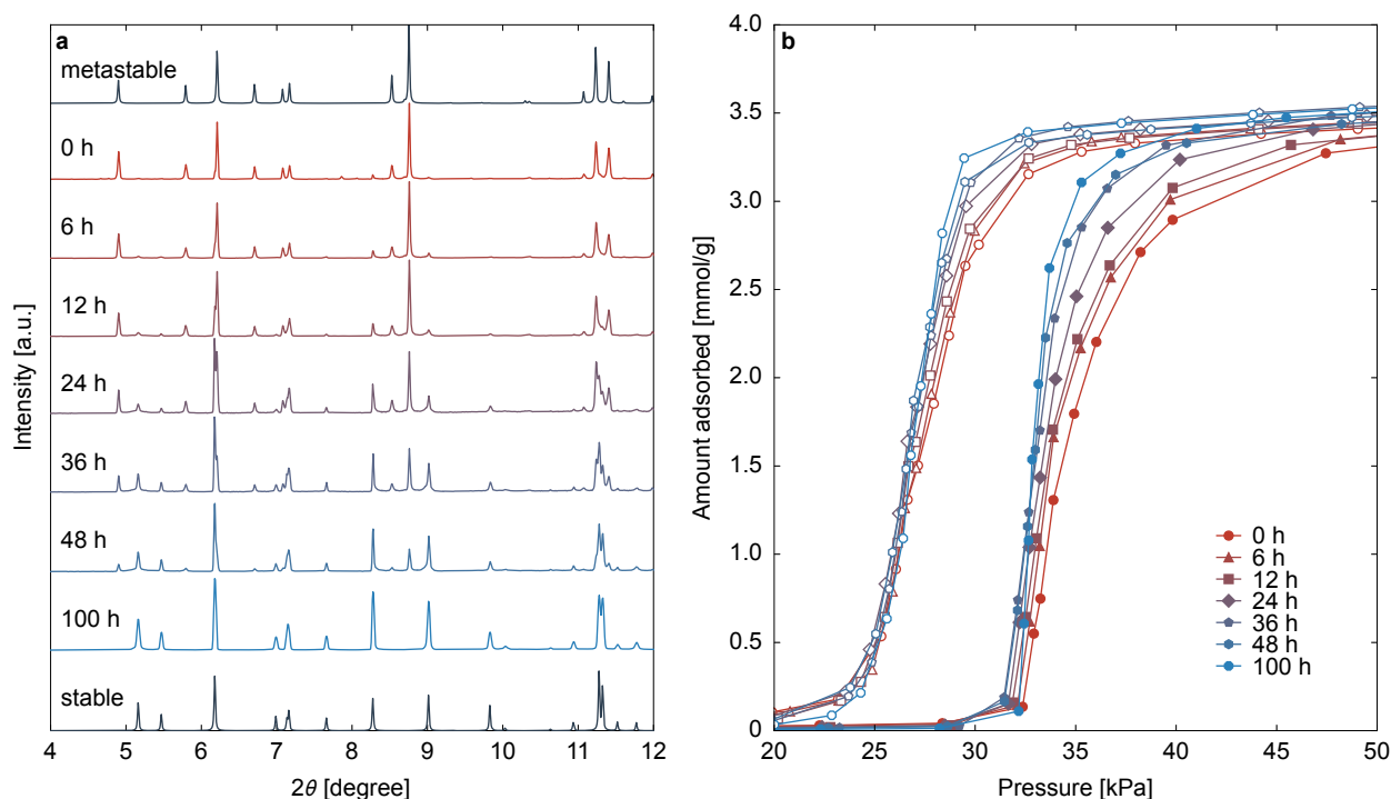
Fig. 2 The impact of aging time on the synthesis at high concentration on (a) the XRD pattern of pre-ELM-11 and (b) the CO 2 adsorption isotherm on ELM-11 at 273 K. The XRD patterns were measured at \lambda = 0.0799932 nm.
