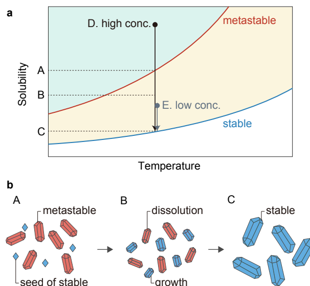
Fig. 4 Schematics of the solvent-mediated phase transformation of pre-ELM-11 during aging process.
