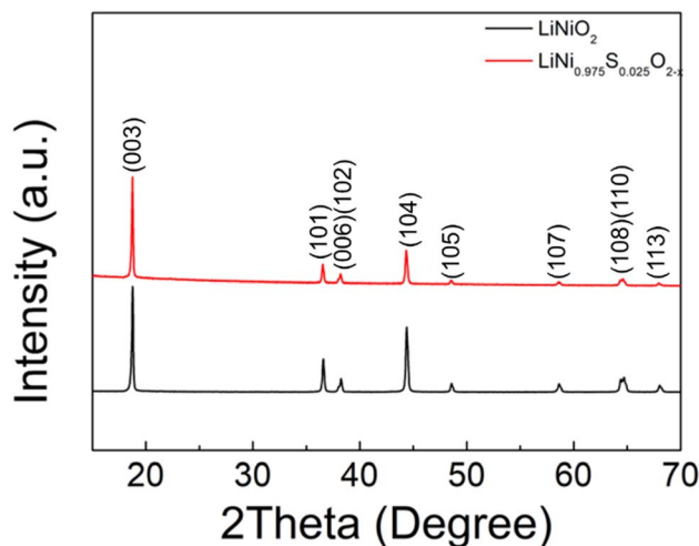
Fig. 1 XRD patterns of LiNiO 2 and S doped LiNiO 2 (solid state synthesis route).
