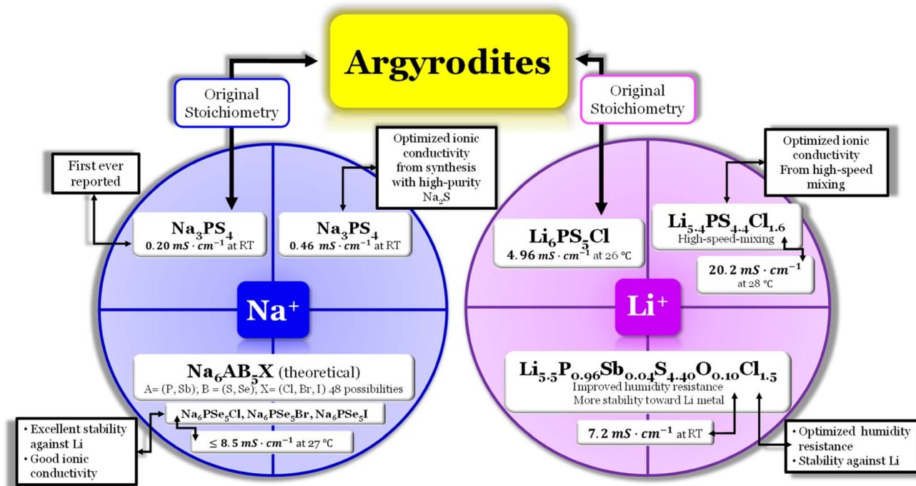
Fig. 6 Arggyrodite summary scheme, \text{Li}_6\text{PS}_5\text{Cl} , 14 \text{Li}_{5.4}\text{PS}_{4.4}\text{Cl}_{1.6} , 30 \text{Li}_{5.5}\text{P}_{0.96}\text{Sb}_{0.04}\text{S}_{4.40}\text{O}_{0.10}\text{Cl}_{1.5} , 83 \text{Na}_3\text{PS}_4 , 84,85 and \text{Na}_6\text{AB}_5\text{X} , A = (P, Sb), B = (S, Se), and X = (Cl, Br, I). 86
