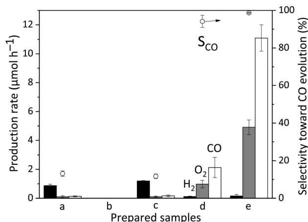
Fig. 6 Results of the photocatalytic reaction tests for \text{CO}_2 reduction with water over the various samples, (a) bare \text{CaTiO}_3 , (b) bare \text{GaOOH} , (c) \text{GaOOH}(1.0)/\text{CTO} , (d) \text{Ag}(1.0)/\text{CTO} , and (e) \text{Ag}(1.0)/\text{GaOOH}(1.0)/\text{CTO} . Production rates of \text{CO} (white bar), \text{H}_2 (black bar), and \text{O}_2 (gray bar) and the \text{CO} selectivity ( S_{\text{CO}}\% , open circles) are shown for each sample. The data were recorded at 3.5 h after the start of photoirradiation.
