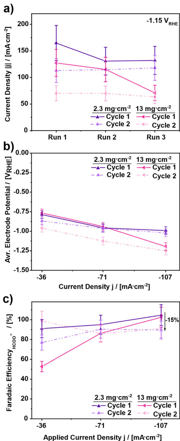
Fig. 3 (a) Evaluation of the cathodic current density at -1.15 V_{RHE} to determine the influence of repeated cycling on the GDE stability for GDE catalyst loadings of 2.3 and 13 mg cm^{-2} . (b) Comparison of the average electrode potential for three different current densities (36, 71 and 107 mA cm^{-2} ). (c) Faradaic efficiency for formate after a run time of 11 min each. (Measurement conditions: batch reactor, 12 ml electrolyte, 1 M KHCO_3 , continuous CO_2 supply of 20 ml min^{-1} , start at room temperature, electrolysis time: 45 min each).
