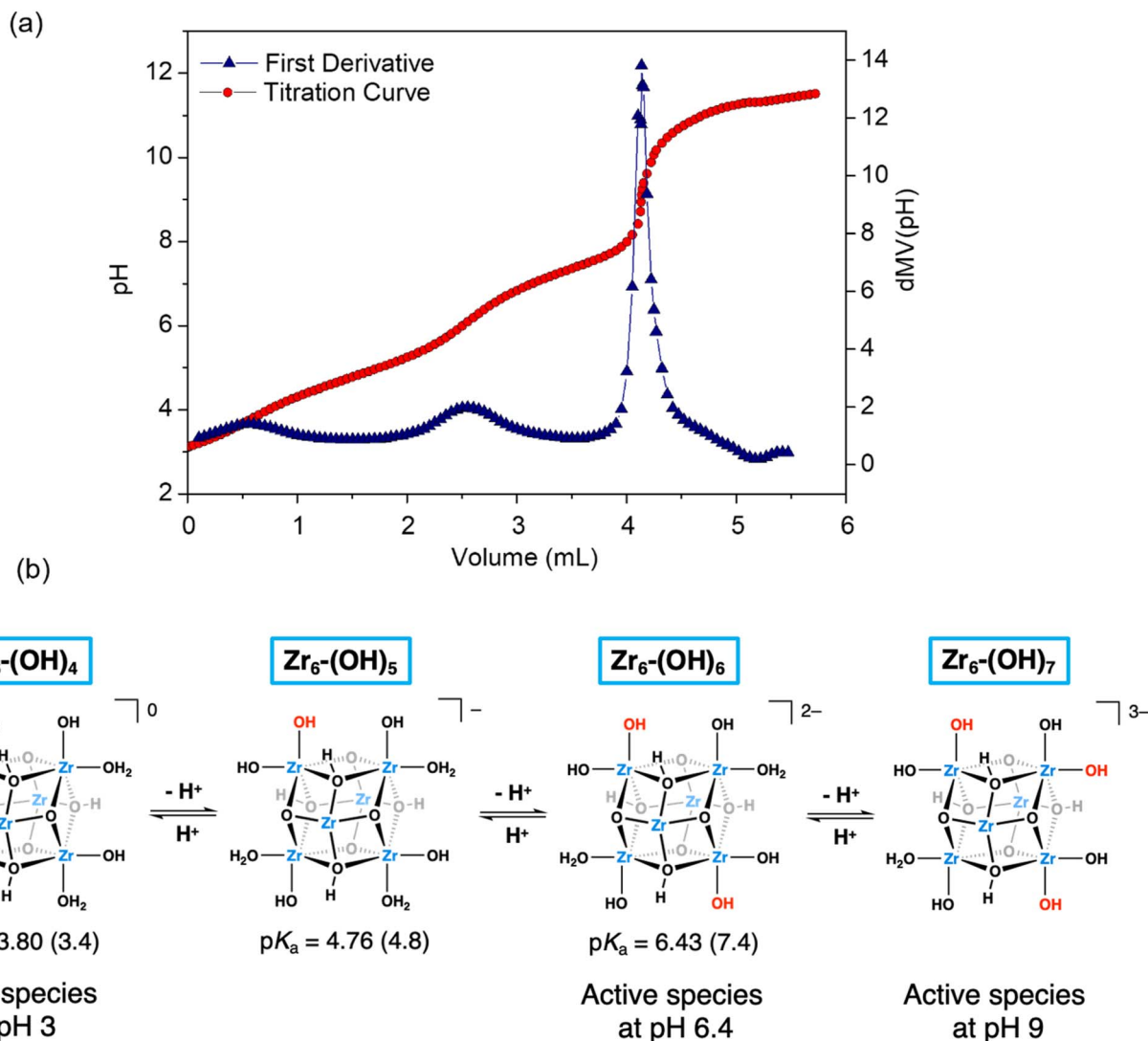
Fig. 6 (a) Zr 6 cluster titration curve (red circles) and its first derivative (blue triangles). Conditions: [Zr 6 ] = 1 × 10 -3 mol L -1 , [KCl] = 0.02 mol L -1 , water (40 mL) p H i = 3.0, p H f = 11.5, titrant KOH – 0.1 mol L -1 ; (b) proposed acid–base equilibria for Zr 6 -(OH) n species. DFT-derived assignment of the experimental pK a values are given in parentheses. Bridging acetate ligands are omitted for clarity. The stability of each species with regard to its structural isomers, which differ in the relative positions of protons, is evaluated in Scheme S3.†
