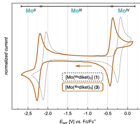
Fig. 3 CV of [\text{Mo}(t^{\text{Bu}}\text{diket})_3] ( 3 ) (1 mM, solid line) and [\text{Mo}^{\text{Me2diket}}_3] ( 1 ) (1 mM, dashed line) in \text{TBAPF}_6/\text{MeCN} (0.1 M) at a scan rate of \nu = 100 \text{ mV s}^{-1} .
