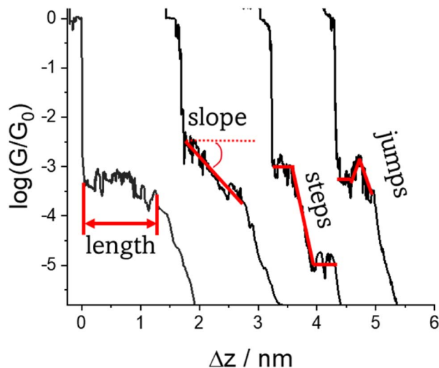
Fig. 7 Conductance–distance traces (displaced along the \Delta z axis for clarity) with examples of different features (length, slope, steps and jumps) that characterise junction formation and evolution events.
