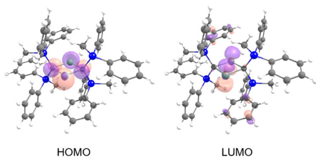
Fig. 9 Kohn–Sham orbitals of 6 .
