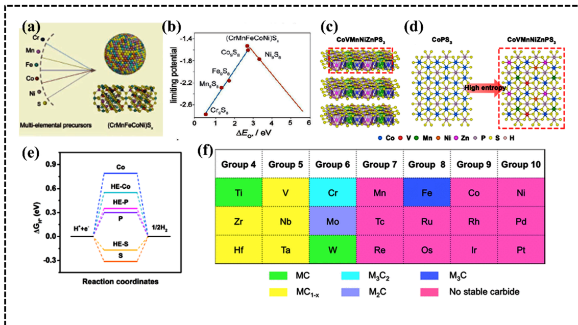
Fig. 10 (a) Schematic demonstrating the structure and activity of high-entropy metal sulfide ((CrMnFeCoNi) x S x ) nanoparticles. (b) Calculated catalytic activity volcano plot. Reproduced with permission. 147 Copyright 2021, Wiley-VCH. (c) DFT calculation in the edge mode; crystal structure of the monoclinic structure, (d) structural polymorphs of CoPS 3 and CoVMnNiZnPS 3 along the top views, and (e) hydrogen evolution reaction free-energy diagram of the corresponding edge sites. Reproduced with permission. 155 Copyright 2022, American Chemical Society. (f) Elements in the synthesized high-entropy carbide (HEC) system. Reproduced with permission. 166 Copyright 2013, American Chemical Society.
