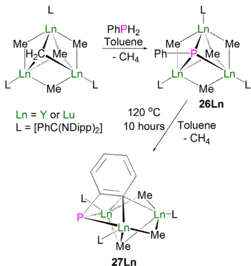
Scheme 9 Synthesis of Lu- and Y-phosphinidide complexes 26Ln–27Ln .
