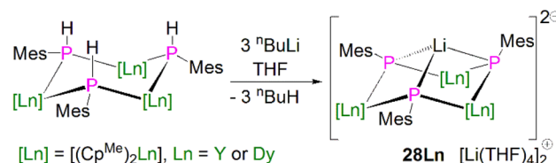
Scheme 10 Synthesis of Y- and Dy-phosphinidide complexes 28Ln .
