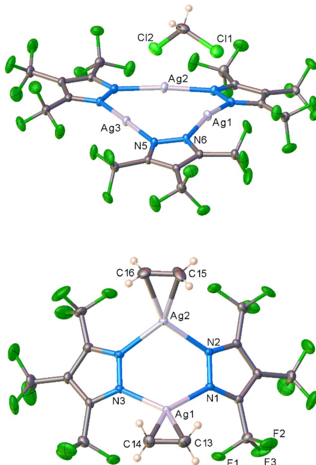
Fig. 2 Molecular structure of [\text{Ag-CF}_3]_3 \cdot \text{CH}_2\text{Cl}_2 (top) and [\text{Ag-CF}_3]_3 \cdot (\text{C}_2\text{H}_4)_2 (bottom) obtained from solution process and single crystal X-ray diffraction studies.
