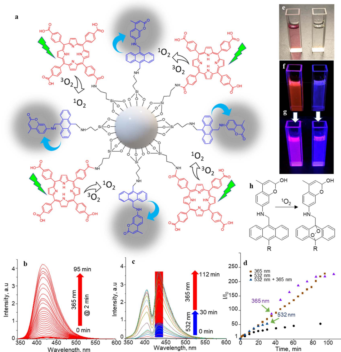
Fig. 2 1 O 2 generation, sensing, and releasing. (a) The SS-MSN structure and its 1 O 2 generation and sensing processes. (b and c) FL spectra ( \lambda_{\text{ex}} = 320 \text{ nm} ) of (b) 4 ( 10 \mu\text{M} in \text{CH}_3\text{CN} , without TCPP) before and after irradiation at 365 nm for 95 min at 2 min intervals. (c) 4 ( 10 \mu\text{M} in \text{CH}_3\text{CN} ) in a TCPP solution ( 5 \mu\text{M} ) before and after photoactivation at 532 nm ( 50 \text{ mW cm}^{-2} ) for 30 min (blue bar) followed by UV illumination (365 nm, 5 \text{ mW cm}^{-2} ) for 82 min (red bar) showing the sensitization-sensing process followed by UV-induced 1 O 2 releasing/AMA oxidation. (d) Time-trace of the peak FL intensities at different photoirradiation conditions in (b) and (c). (e–g) Photographs of (left) a mixture of 4 and TCPP and (right) 4 (e) under visible light before photoactivation, (f) <1 min under UV light after 30 min 532 nm laser irradiation ( 50 \text{ mW cm}^{-2} ) for 30 min, and (g) ca. 5 min under UV light after 30 min 532 nm laser irradiation ( 50 \text{ mW cm}^{-2} ). (h) A scheme of 1 O 2 reaction on the sensor.
