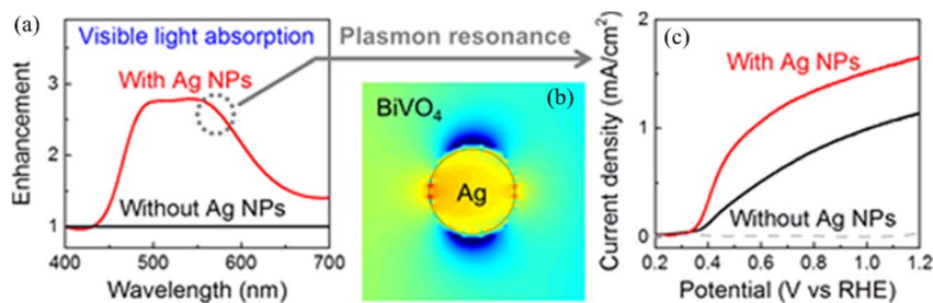
Fig. 8 Applications of plasmon-enhanced photocatalytic water splitting with a Ag NP-impregnated \text{BiVO}_4 composite: (a) absorption enhancement of \text{BiVO}_4 with and without Ag NPs; (b) simulated light absorption distribution of \text{BiVO}_4 with a Ag NP; and (c) current density as a function of the potential of \text{BiVO}_4 with and without Ag NPs. 68 Reproduced from ref. 68 with permission from the American Chemical Society, copyright [2018].
