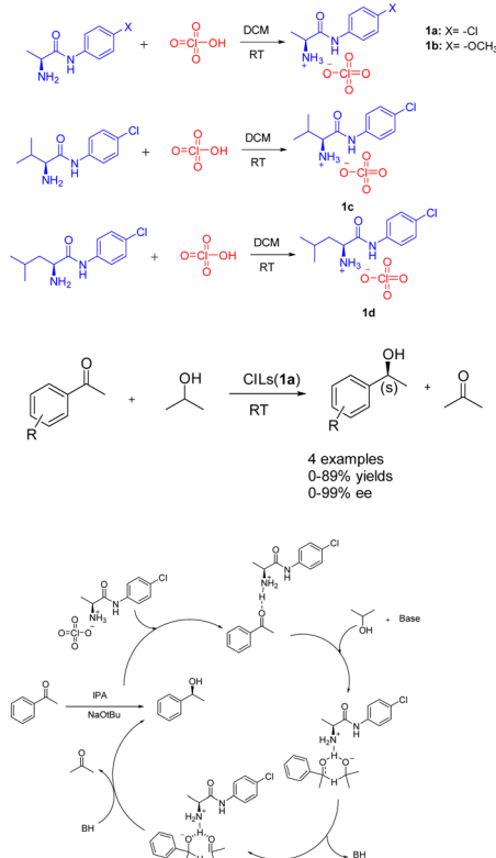
Scheme 1 Synthesis of amide-modified chiral ionic liquids and asymmetric ATH reaction of acetophenone and its mechanism.
