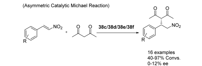
Scheme 38 Synthesis and application of chiral ureamine bifunctional catalysts supported by silica in asymmetric reactions.
