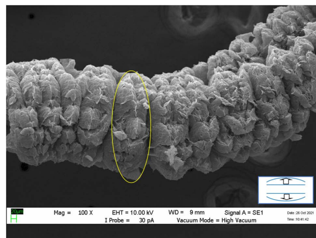
Fig. 1 SEM photographs of expanded graphite. Reprinted with permission from ref. 75.
