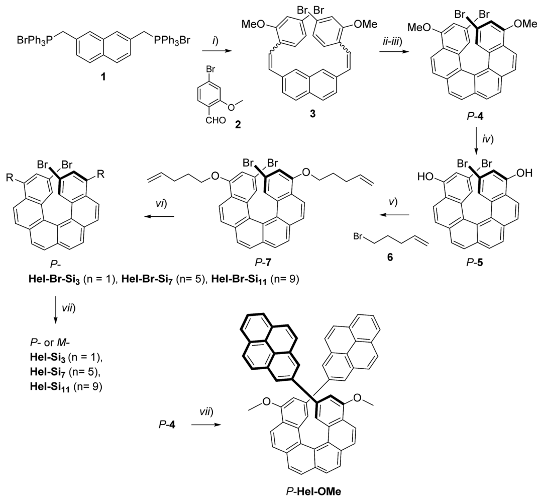
Scheme 1 Synthetic route to enantiopure oDMS end-functionalized carbo[6]helicenes P - Hel-Si n and Hel-OMe . (i) n -BuLi, rt, Ar, 3 h, 94%; (ii) I 2 , toluene, Ar, propylene oxide, hν , 7 h, 61%; (iii) chiral HPLC resolution (see the ESI†); (iv) BBr 3 , CH 2 Cl 2 , rt, Ar, 12 h; (v) K 2 CO 3 , DMF, Ar, 65 °C, overnight, 67%; (vi) Karstedt's catalyst, Si (2+n) H, CH 2 Cl 2 , rt, Ar, 12 h, 73% ( n = 1 ), 59% ( n = 5, 9 ); (vii) pyrene-2-boronic acid, Pd(PPh 3 ) 4 , Na 2 CO 3 , DMF, 80 °C, Ar, 12 h, 43–55%. The same strategy was used for the M enantiomers. The detailed R substituents can be seen in Fig. 1.
