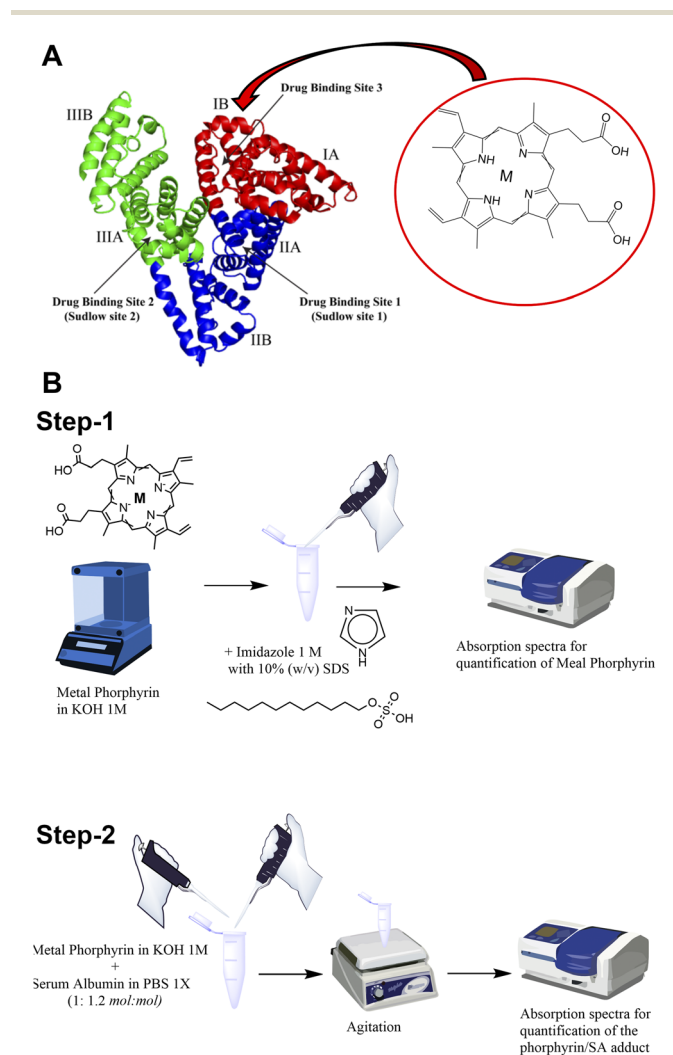
Scheme 1 (A) Schematic illustration of the interaction of serum albumin with protoporphyrin IX (M = Mn(III) or Fe(III) or Zn(II)). (B) Scheme of the preparation of metal porphyrin serum albumins (step-1: UV-vis spectrophotometric quantification of metal porphyrin; step-2: preparation and quantification of metal porphyrin serum albumins).
