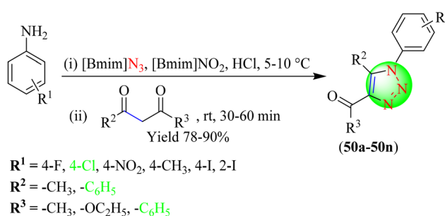
Scheme 54 Synthesis of 1,2,3-triazoles ( 50a–50n ) using ILs as an azide source and reaction medium.
