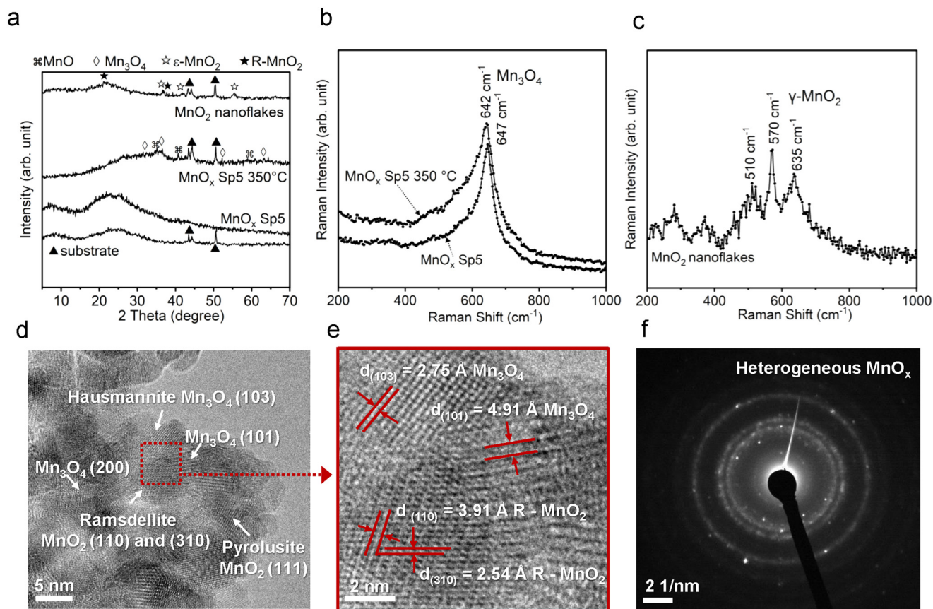
Fig. 2 a) XRD diffraction patterns of as-prepared spark-ablated manganese oxide ( \text{MnO}_x Sp5), calcined at 350\text{ }^\circ\text{C} ( \text{MnO}_x Sp5 350\text{ }^\circ\text{C} ) and sol-gel prepared \text{MnO}_2 nanoflakes. b) Raman spectra of as-prepared ( \text{MnO}_x Sp5) and calcined ( \text{MnO}_x Sp5 350\text{ }^\circ\text{C} ) spark-ablated samples. c) Raman spectrum of the sol-gel prepared \text{MnO}_2 nanoflake sample. d) HRTEM images of \text{MnO}_x Sp showing hausmannite, ramsdellite and pyrolusite crystalline structures; e) measured planar spacing with the determination of miller indices ( hkl ). f) Selected area electron diffraction (SAED) image of heterogeneous \text{MnO}_x Sp5.
