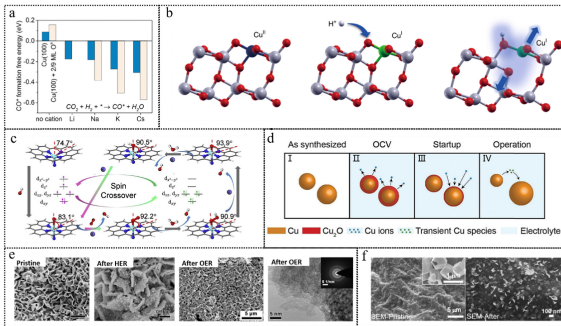
Fig. 5 (a) CO* formation free energy calculated in the absence and presence of Li + , Na + , K + , and Cs + on bare Cu(100) and Cu(100) with 2/9 ML O * . This figure has been reproduced from ref. 46 with permission from American Chemical Society, copyright 2018. (b) Schematic representation of the variation in the chemical state of Cu during photocatalysis. This figure has been reproduced from ref. 47 with permission from Nature, copyright 2019. (c) Structure and dynamics of the N-FeN 4 C 10 moiety in the ORR with optimized geometries (the angles represent the deviation of iron from the N 4 -plane). This figure has been reproduced from ref. 48 with permission from Elsevier, copyright 2020. (d) Schematic representation of the catalyst reconstruction process: (I) the as-synthesized metallic Cu NPs, (II) the catalyst oxidation and dissolution of Cu ions into the electrolyte, (III) the redeposition of dissolved ions onto the catalyst when a reducing potential is applied, and (IV) the dissolution of smaller particles into transient species, whose nature remains unknown to date, that contribute to the growth of larger nanoparticles under a constant applied potential during cell operation. This figure has been reproduced from ref. 49 with permission from Wiley-VCH, copyright 2020. (e) SEM images and a high-resolution TEM image of pristine FeS/IF, FeS/IF after the HER and FeS/IF after the OER. This figure has been reproduced from ref. 50 with permission from Elsevier, copyright 2018. (f) SEM images of the as-prepared (pristine) CoS x /NGF and the CoS x /NGF after the OER. This figure has been reproduced from ref. 51 with permission from American Chemical Society, copyright 2018.
