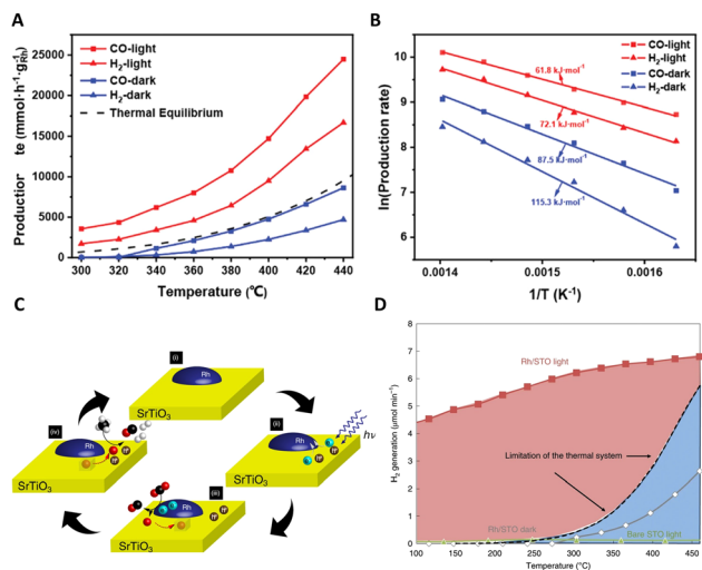
Fig. 5 (A) and (B) Production rates and apparent activation energy of \text{H}_2 and CO under irradiation or heating over Rh/LaNiO 3 . These figures have been reproduced from ref. 108 with permission from John Wiley & Sons, copyright 2023. (C) Tentative mechanistic aspects of the photocatalytic DRM by Rh/STO. (D) The temperature dependence of DRM activity under dark and light irradiation conditions. These figures have been reproduced from ref. 109 with permission from Springer Nature, copyright 2020.
