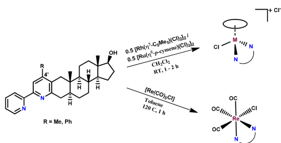
Chart 2 Reaction scheme for the synthesis of complexes 1–6 . The composition of complexes 1–6 is given in Table 1.
