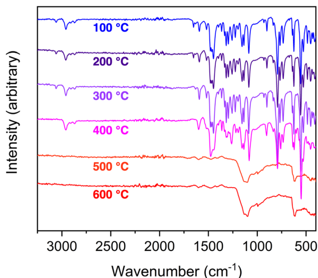
Fig. 3 Infrared spectra collected for [(\text{Fe}_4\text{OHsc4a})_6(\text{BTtri})_8]^{6-} as a function of activation temperature. Consistent with TGA data, the cage displays minimal structural degradation up to an activation temperature of at least 400 °C.
