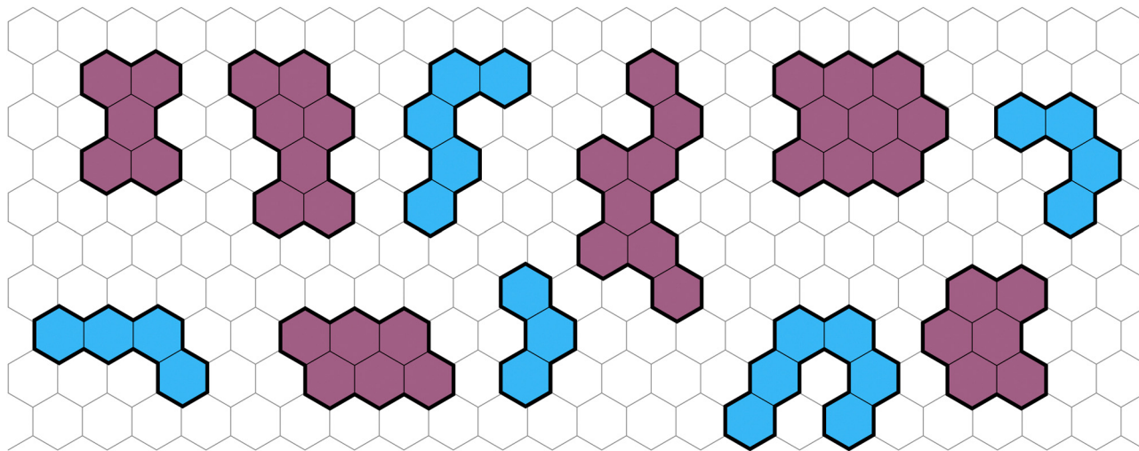
Fig. 1 Representative examples of PBHs on a background of a hexagonal grid, cc-PBHs are colored in blue and pc-PBHs are colored in purple.
