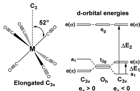
Fig. 6 Trigonal distortion applied to M(CO) 6 compounds and relationship between the sense of splitting of the t 2g orbitals and the sign of the e_{\pi} parameter.
