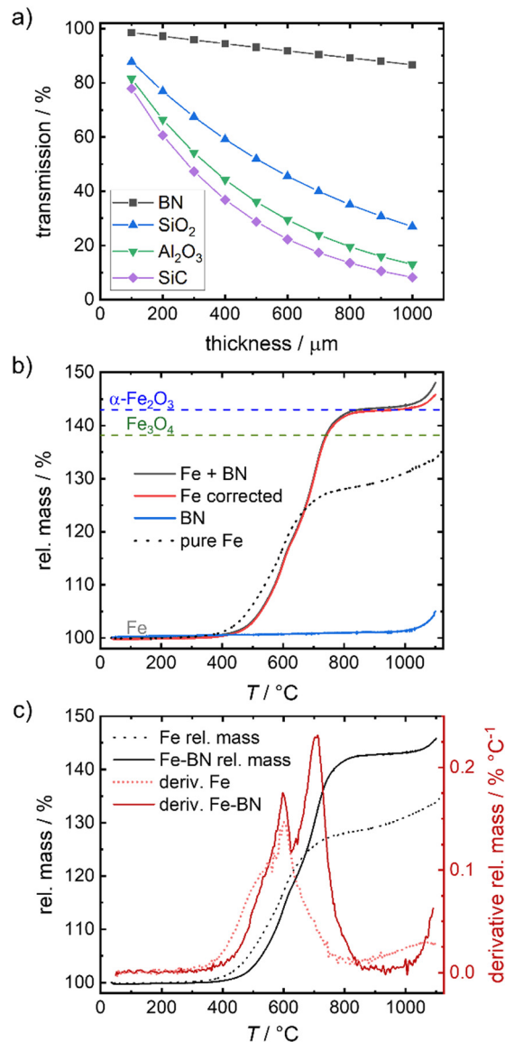
Fig. 3 Relative transmission of \gamma -radiation of 14.4 keV through different thicknesses associated for different dilution agents 54 (a), TGA of Fe mixed with BN (b) and related derivative (10 K min -1 , air) (c) in comparison to the pure iron sample. In (b) Fe corrected corresponds to the rel. mass of Fe + BN mathematically corrected for the rel. mass of BN (in the given mass fractions). The dashed lines in (b) indicate the mass gain assigned to a full oxidation to Fe 3 O 4 and \alpha -Fe 2 O 3 .
