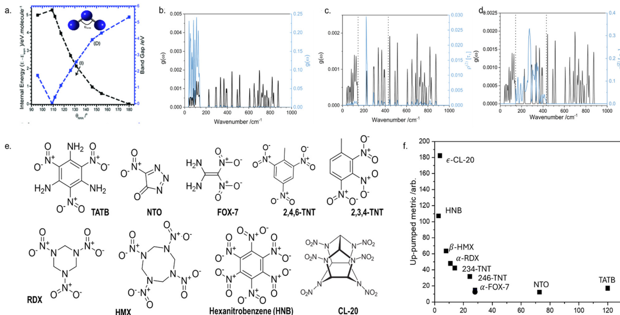
Fig. 5 Initiation of mechanochemical reaction through vibrational excitation. (a) Transient, dynamic metallisation achieved in crystalline NaN 3 through excitation of the azido anion bending mode. (b)–(d) Initial mechanical excitation of low frequency vibrations and subsequent energy transfer to higher frequency molecular vibrations. In each case, the fundamental frequencies are shown in black, and the associated vibrational populations are shown in blue. (b) Initial excitation following mechanical insult, (c) and (d) step-wise transfer of vibrational energy into higher frequency vibrations. (e) Molecular diagrams for the EMs whose mechanochemical reactivity was studied by phonon up-pumping. (f) Semi-quantitative prediction of EM mechanochemical reactivity, with experimental values shown on the x axis and predicted ordering plotted on the y axis. Data are taken from ref. 58.
